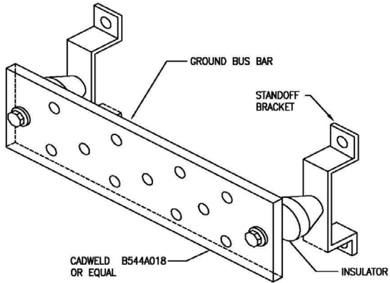
ISOMETRIC ELEVATION
