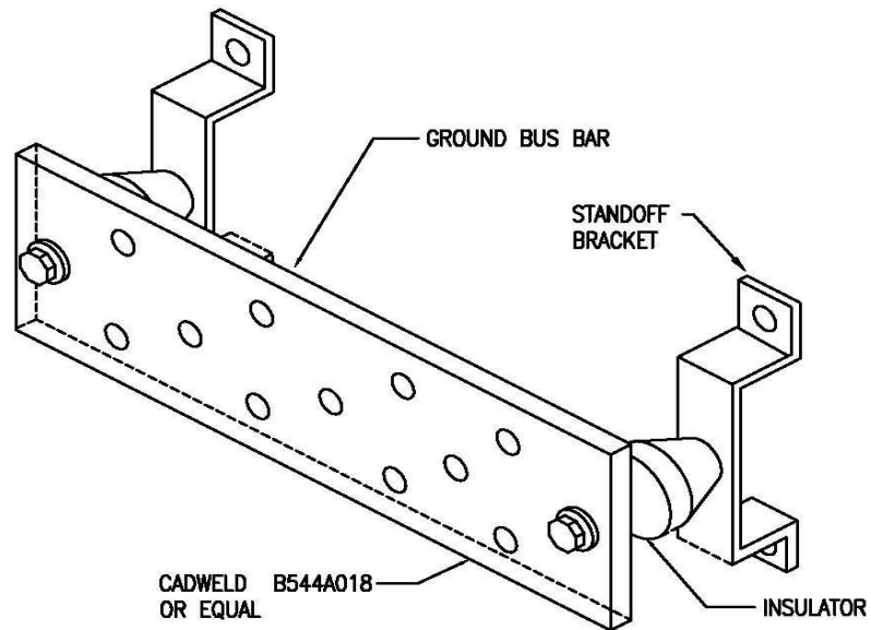
ISOMETRIC ELEVATION
